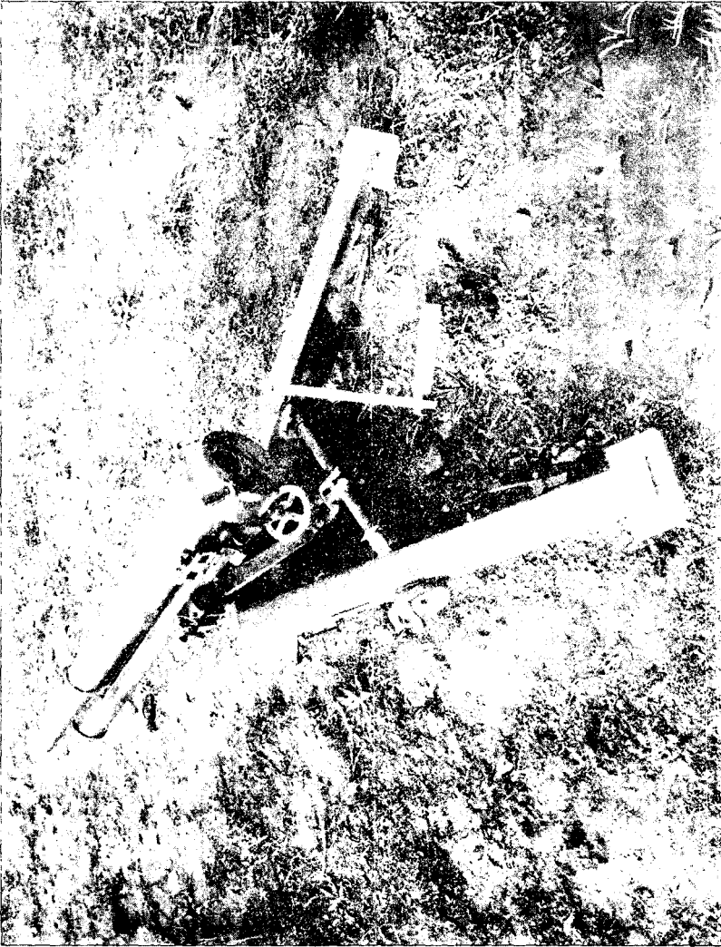
FIGURE 4. - GUN, 37-MM, M1916, ON CARRIAGE, M1916A2.
