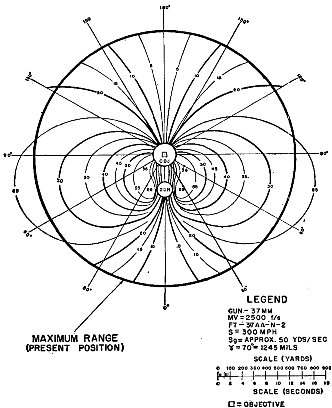
FIGURE 26.—Lateral lead chart, gun-objective distance 300 yards.
