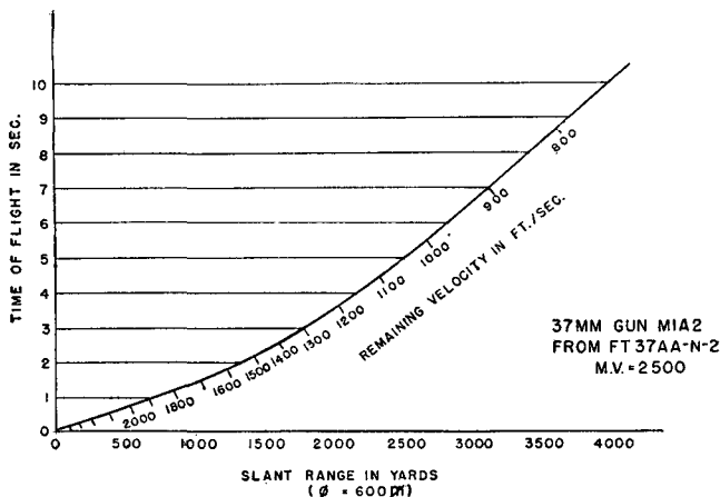
FIGURE 2.—Relation of remaining velocity to time of flight.
