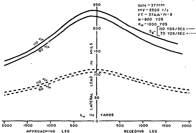
FIGURE 66.—Variation in ballistic density, crossing-constant altitude course (lateral lead).
