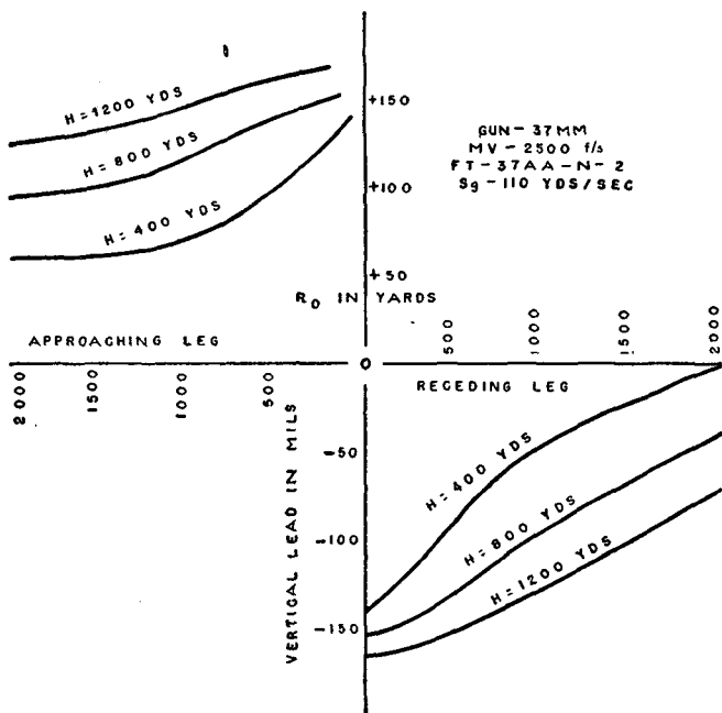
FIGURE 39.—Variation in altitude, coming-constant altitude course.
