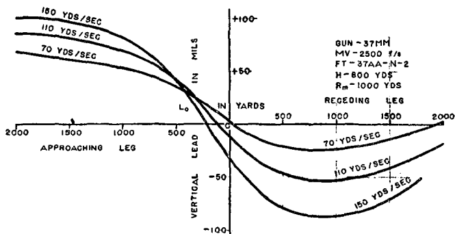
FIGURE 48.—Variation in target speed, crossing-constant altitude course (vertical lead).
