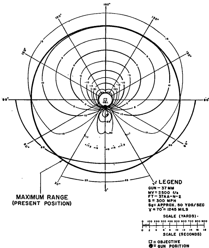
FIGURE 25.—Vertical lead chart, gun-objective distance 100 yards.
