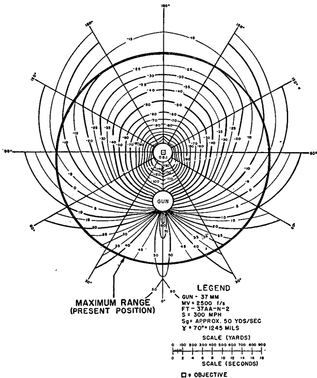
FIGURE 29.—Vertical lead chart, gun-objective distance 500 yards.
