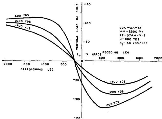
FIGURE 51.—Variation in R_m , crossing-constant altitude course at service speed (vertical lead).
