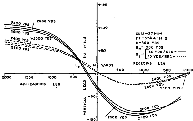
FIGURE 64.—Variation in muzzle velocity, crossing-constant altitude course (vertical lead).
