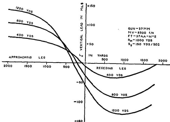
FIGURE 49.—Variation in altitude, crossing-constant altitude course at service speed (vertical lead).
