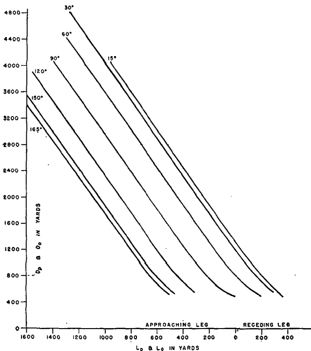
FIGURE 34.—Plot of D_p and L_p curves, gun-objective distance 500 yards.
