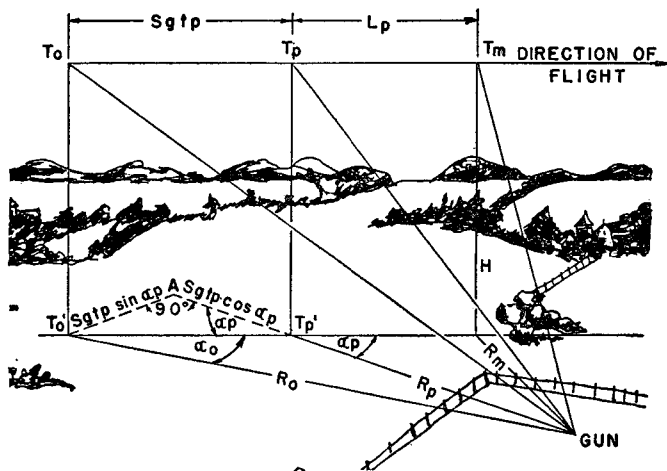
FIGURE 9.—Crossing-constant altitude course.
