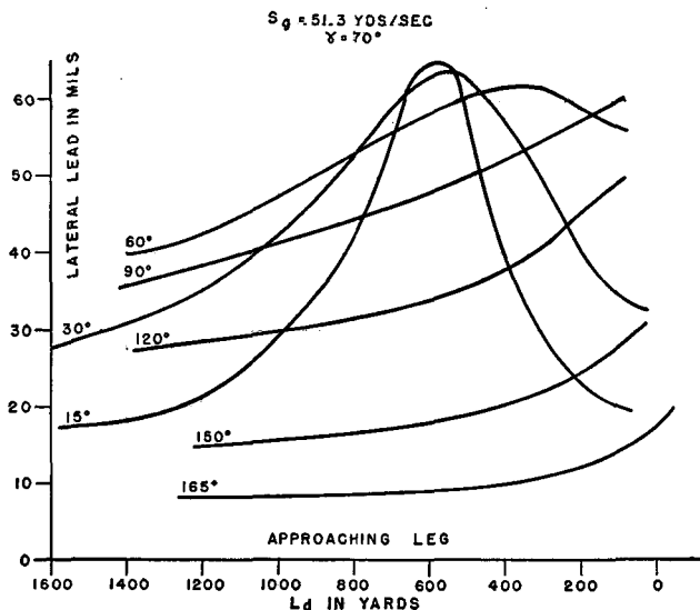
FIGURE 35.—Plot of lateral lead curves against L_d in yards, gun-objective distance 500 yards.
