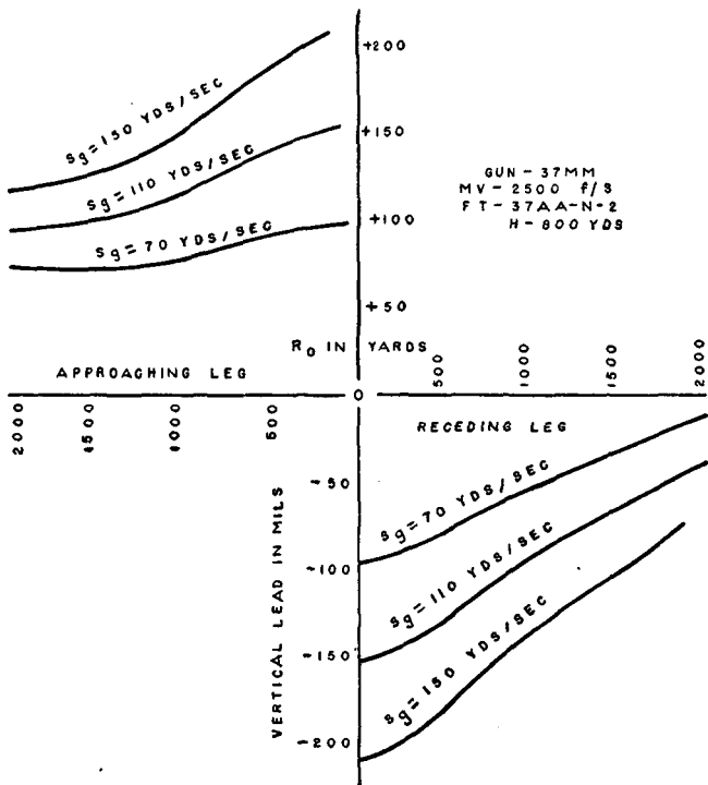
FIGURE 38.—Variation in target speed, coming-constant altitude course.
