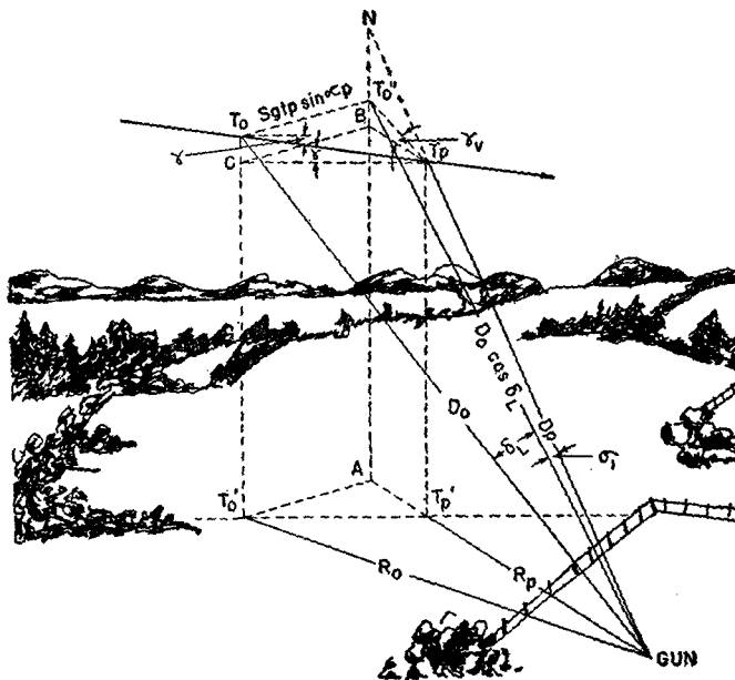
FIGURE 13.—Crossing-diving course, approaching leg.
