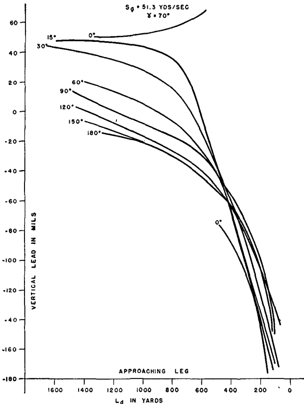
FIGURE 36.—Plot of vertical lead curves against L_d in yards, gun-objective distance 500 yards.
