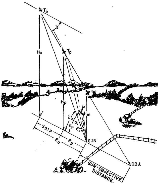
FIGURE 8.—Vertical lead coming-diving course.
