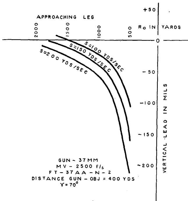
FIGURE 42.—Variation in target speed, coming-diving course, objective in front of gun.
