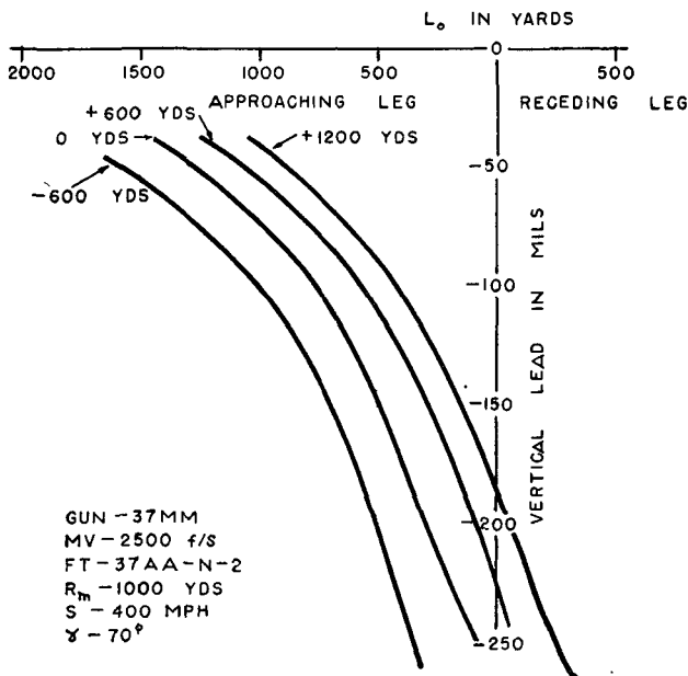
FIGURE 59.—Variation in H_m , crossing-diving course (vertical lead).
