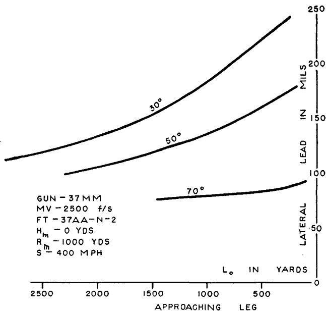
FIGURE 57.—Variation in angle of dive, crossing-diving course (lateral lead).
