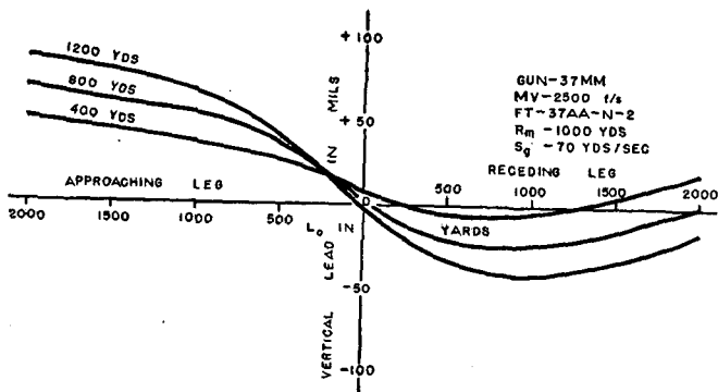
FIGURE 50.—Variation in altitude, crossing-constant altitude course at towed target speed (vertical lead).
