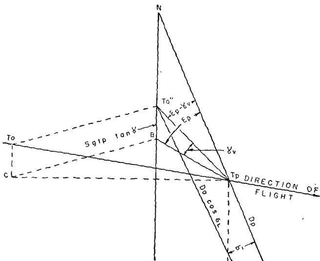
FIGURE 15.—Determination of \sigma_1 , cross-diving course.
