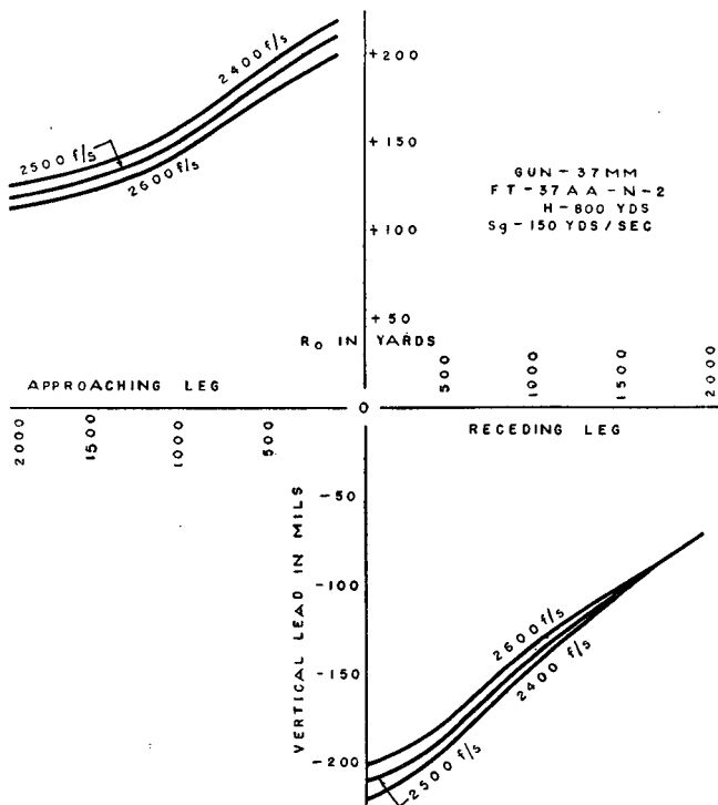
FIGURE 62.—Variation in muzzle velocity, coming-constant altitude course (vertical lead).
