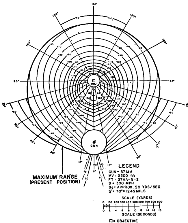
FIGURE 31.—Vertical lead chart, gun-Objective distance 1,000 yards.
