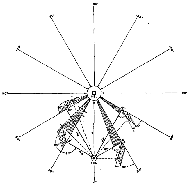
FIGURE 33.—Lead chart showing construction of R_m and H_m .
