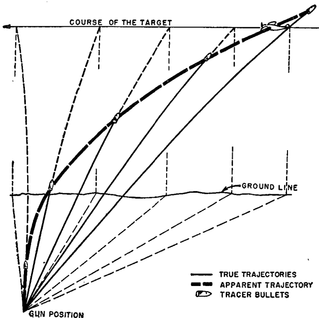
FIGURE 77.—Apparent tracer trajectory.
