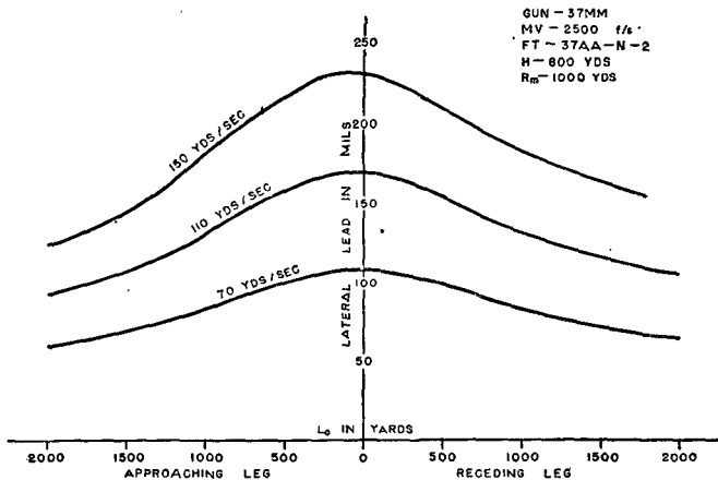
FIGURE 44.—Variation in target speed, crossing-constant altitude course (lateral lead).
