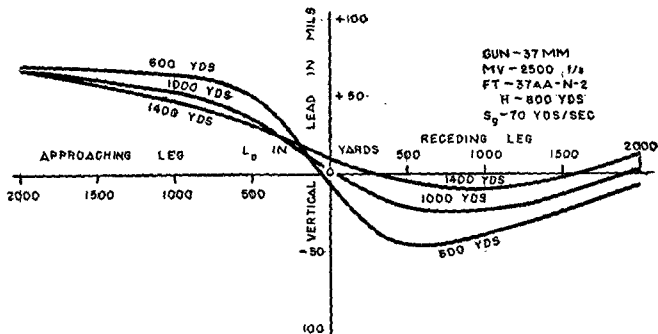
FIGURE 52.—Variation in R_m , crossing-constant altitude course at towed target speed (vertical lead).
