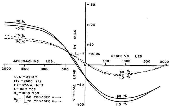
FIGURE 67.—Variation in ballistic density, crossing-constant altitude course (vertical lead).
