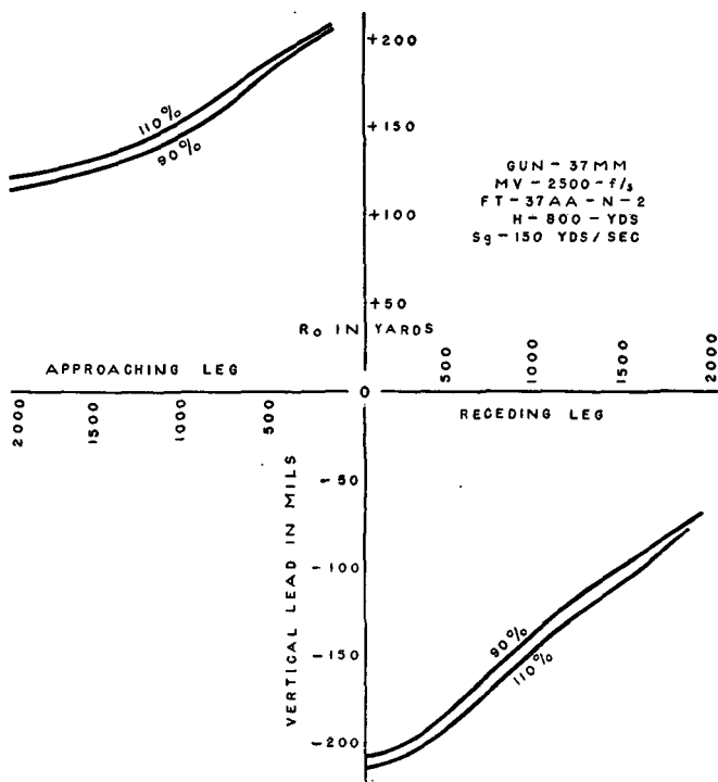
FIGURE 65.—Variation in ballistic density, coming-constant altitude (vertical lead).
