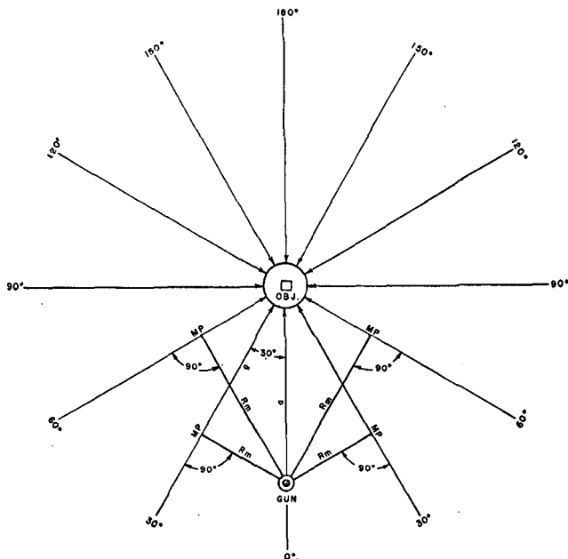
FIGURE 32.—Lead chart showing construction of R_m .
