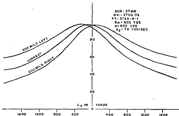
FIGURE 47.—Effect on lateral lead of incorrect estimation of angle of approach, crossing-constant altitude course.
