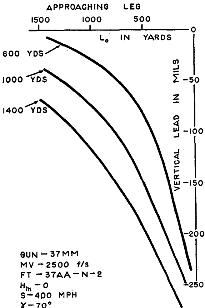
FIGURE 60.—Variation in R_m , crossing-diving course (vertical lead).
