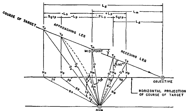
FIGURE 6.—Elements of data for crossing-diving course.
