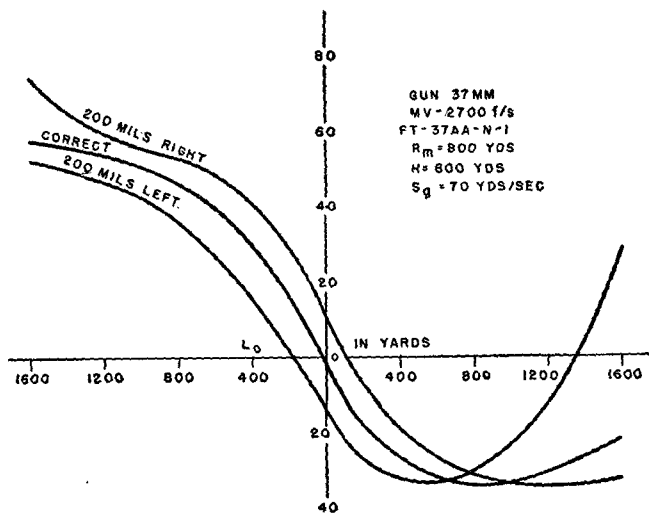
FIGURE 53.—Effect on vertical lead of incorrect estimation of angle of approach, crossing-constant altitude course.
