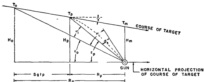
FIGURE 4.—Elements of data for coming-diving course (vertical plane containing gun, T_o , T_p , and T_m ).
