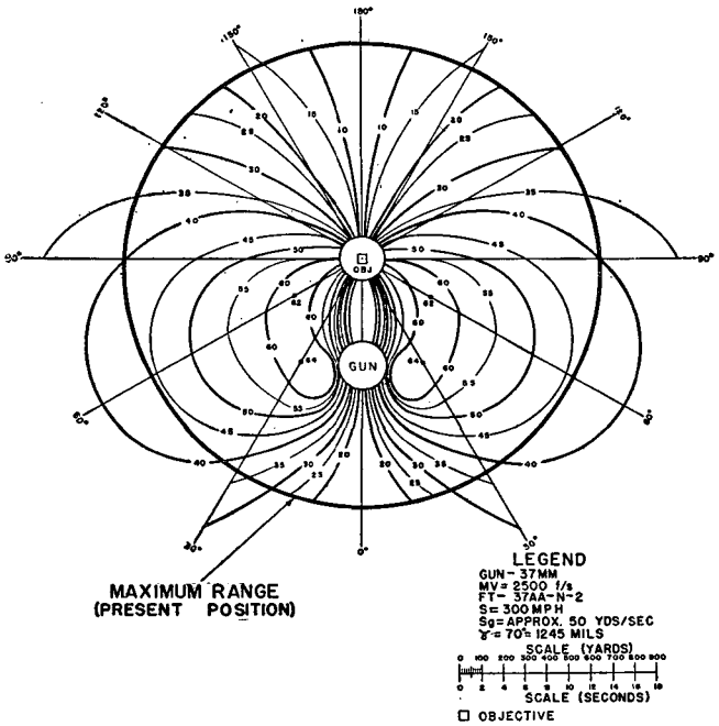
FIGURE 28.—Lateral lead chart, gun-objective distance 500 yards.
