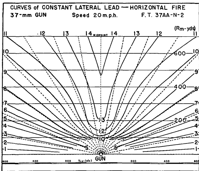
FIGURE 72.—Lateral lead chart, horizontal fire.
