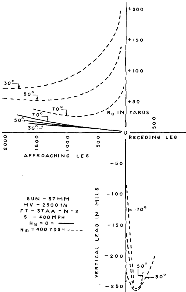
FIGURE 41.—Variation in angle of dive, coming-diving course.
