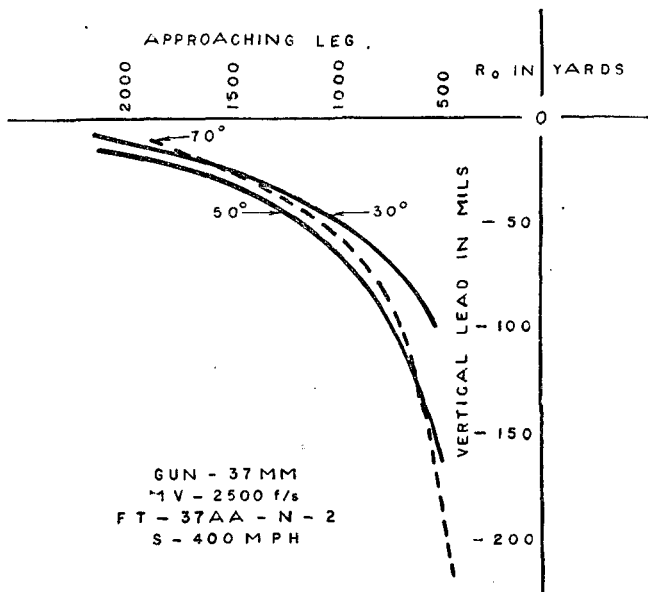
FIGURE 43.—Variation in angle of dive, coming-diving course, objective 400 yards in front of gun.
