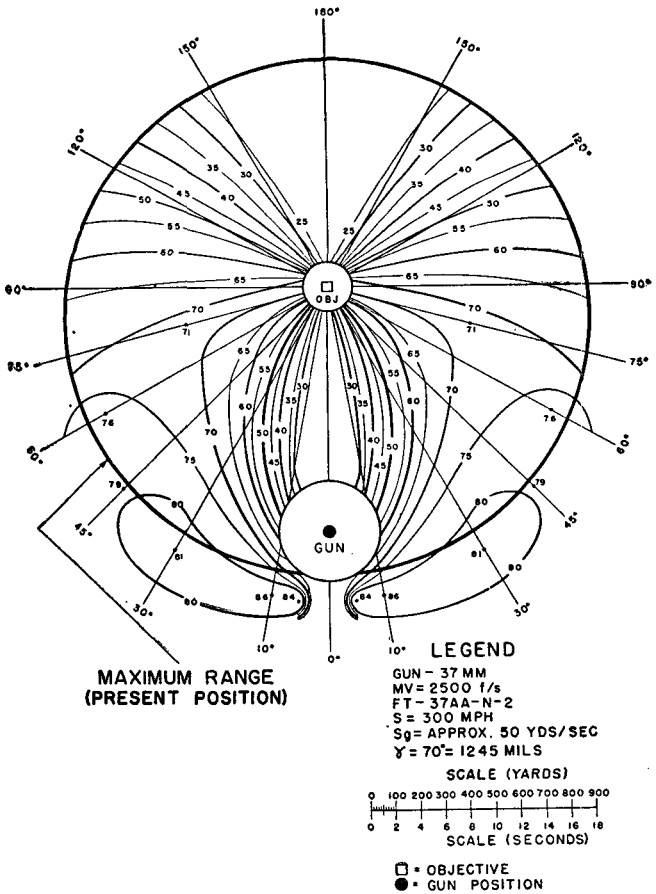
FIGURE 30.—Lateral lead chart, gun-objective distance 1,000 yards.
