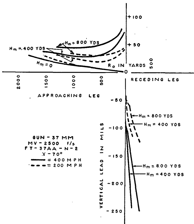
FIGURE 40.—Variation in target speed and in H_m , coming-diving course.
