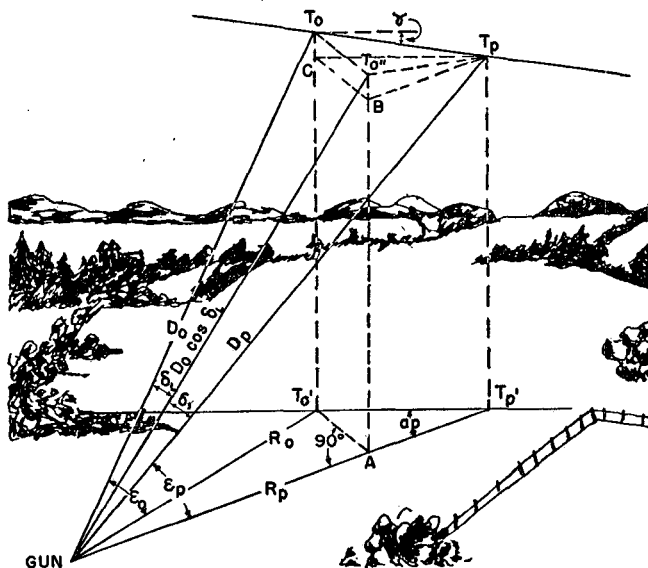
FIGURE 18.—Crossing-diving course, receding leg.
