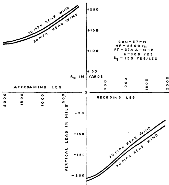
FIGURE 68.—Variation in wind velocity parallel to the trajectory, coming-constant altitude course (vertical lead).
