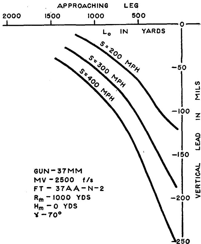
FIGURE 58.—Variation in target speed, crossing-diving course (vertical lead).
