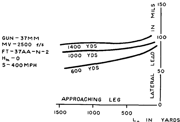
FIGURE 56.—Variation in R_m , crossing-diving course (lateral lead).
