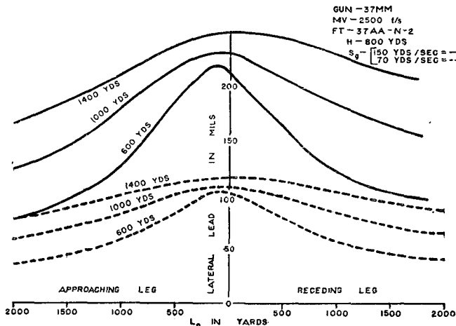
FIGURE 46.—Variation in horizontal range to midpoint, crossing-constant altitude course (lateral lead).
