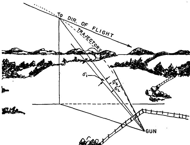
FIGURE 17.—Determination of \sigma_L , approaching leg.
