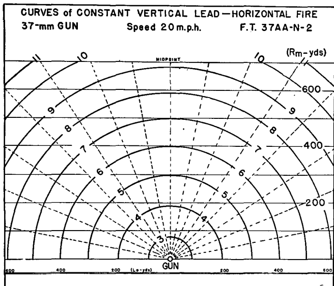
FIGURE 73.—Vertical lead chart, horizontal fire.
