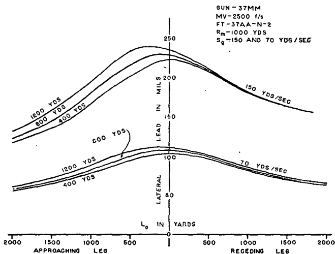
FIGURE 45.—Variation in altitude, crossing-constant altitude course (lateral lead).
