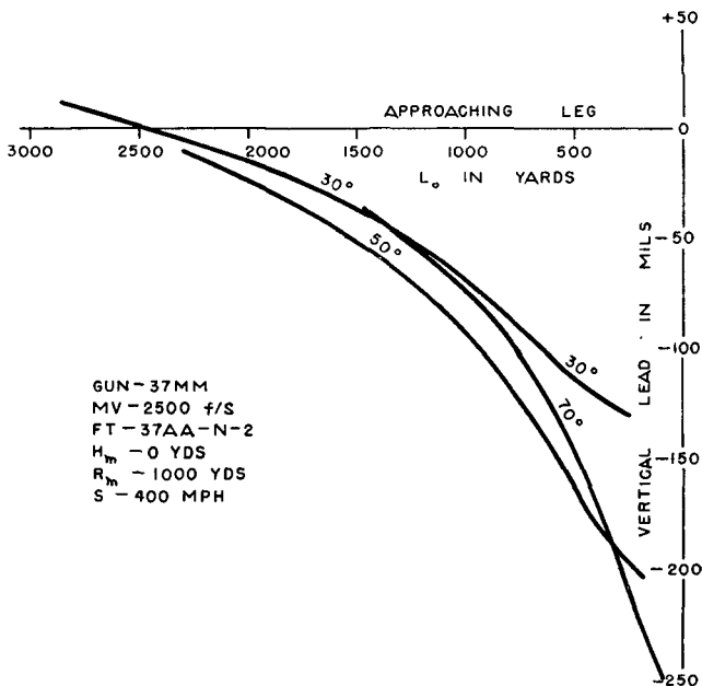
FIGURE 61.—Variation in angle of dive, crossing-diving course (vertical lead).
