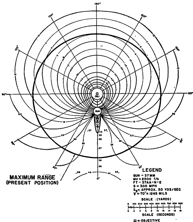
FIGURE 27.—Vertical lead chart, gun-objective distance 300 yards.
