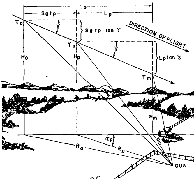
FIGURE 12.—Crossing-diving course.
