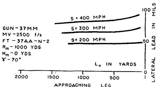
FIGURE 54.—Variation in target speed, crossing-diving course (lateral lead).
