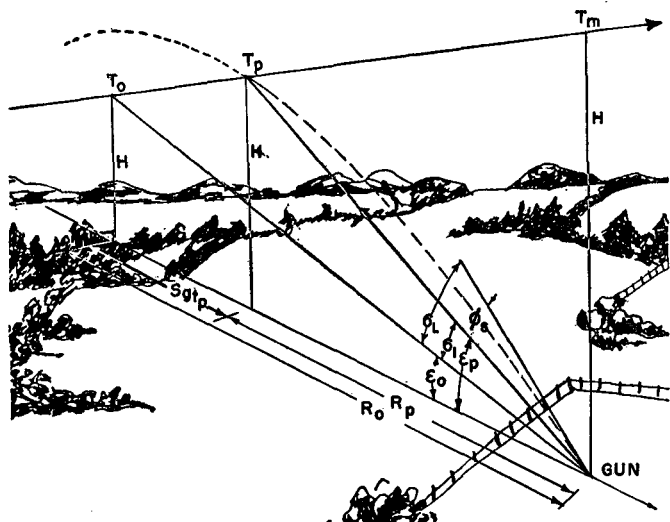
FIGURE 7.—Vertical lead, coming-constant altitude course.
