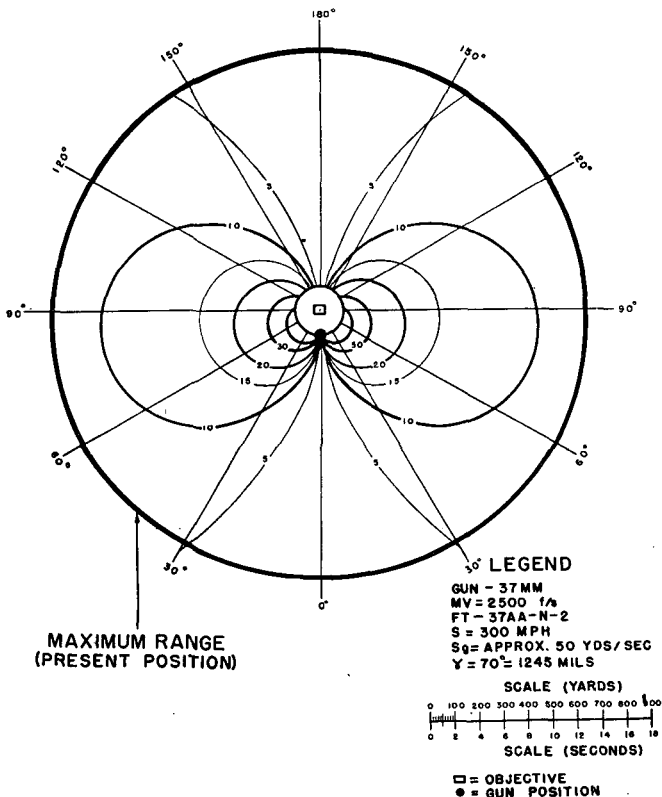
FIGURE 24.—Lateral lead chart, gun-objective distance 100 yards.
