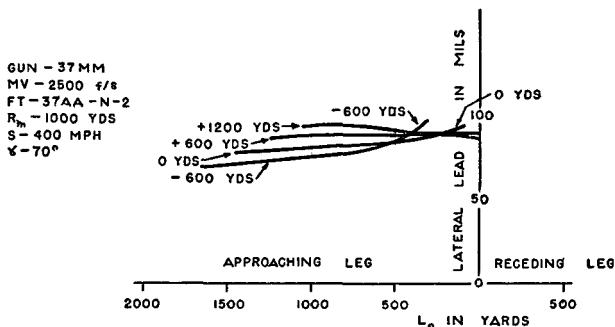
FIGURE 55.—Variation in H_m , crossing-diving course (lateral lead).
