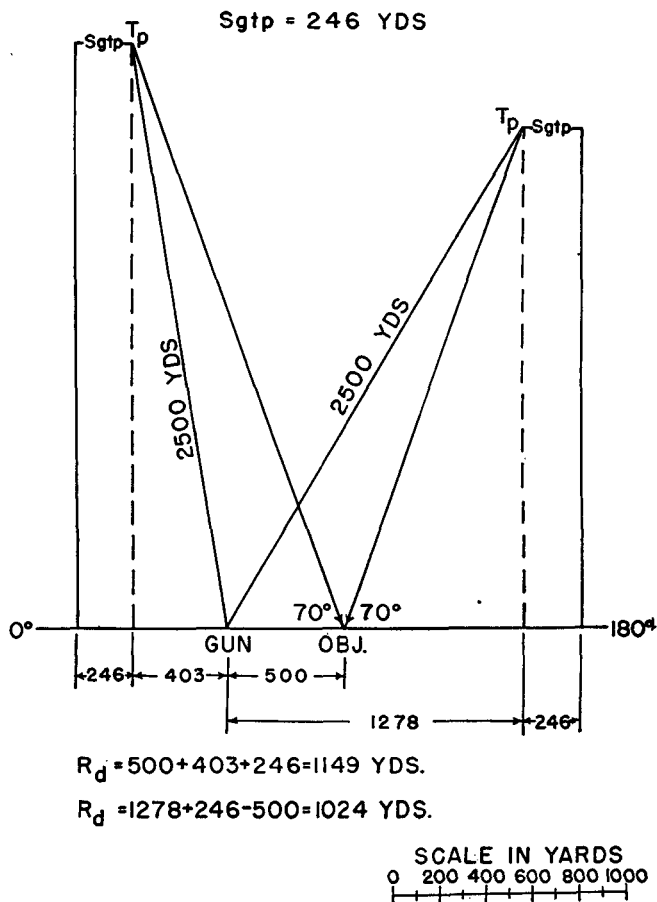
FIGURE 37.—Coming-diving target, vertical plane, gun-objective distance, 500 yards.
