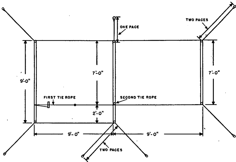
Figure 41. Screen, latrine, top view.
