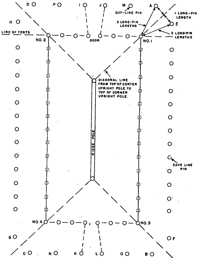
Figure 22. Method of placing pins to pitch tents.
