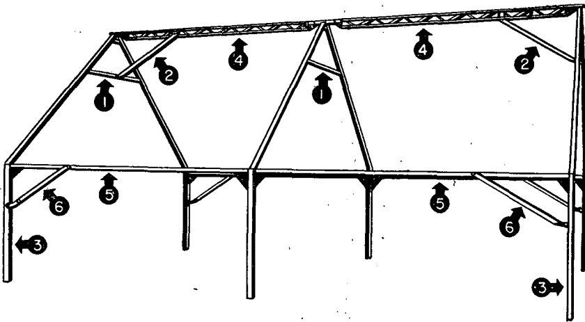
Figure 34. Component parts of frame, tent, maintenance shelter, stock No. 24-F-675.
