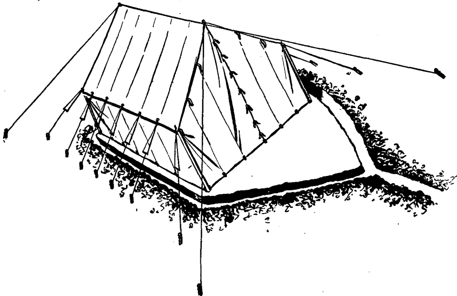
Figure 44. An outlet trench is constructed.
