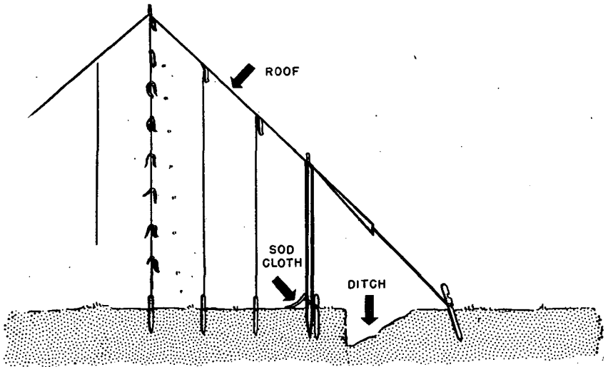
Figure 43. Cross-sectional view of tent trench.
