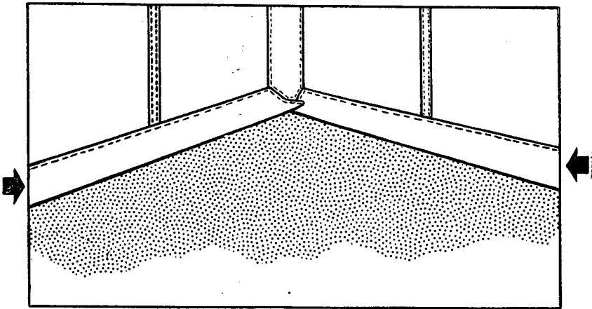
Figure 50. The sod cloth.
