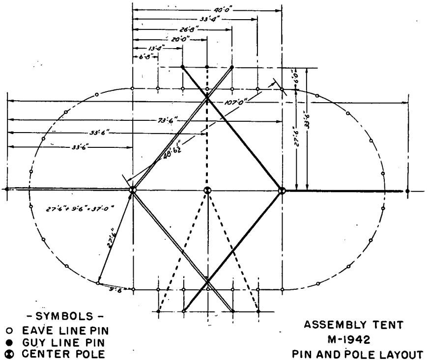
Figure 30. Pin and pole lay-out.
